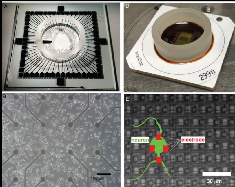
Neurons grown on Microelectrode Array (MEA)
